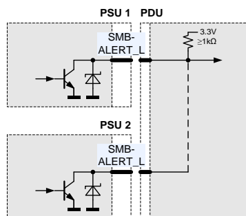
Figure 16. SMBALERT_L connection
