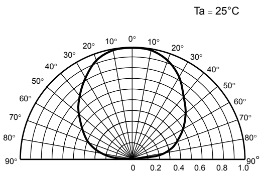
Radiation pattern (typ.)
