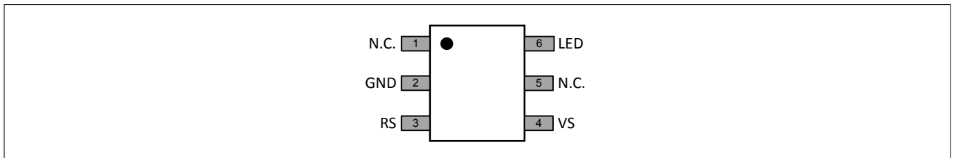
Figure 2 Pinout BCR430
