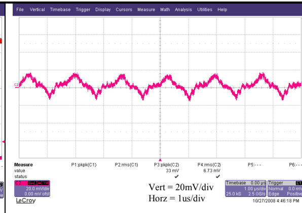
Vo=1.8V Typical Input Ripple at nominal Input Voltage and full load at Ta=25 degrees. Input capacitors 2 x 22µF ceramic
