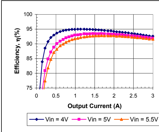
V_o = 3.3V
