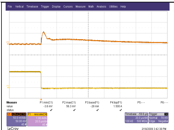
Vo=1.8V Typical output voltage transient response to load step from 100% to 50% of full load with output current slew rate of 10A/uS. (Cext = 1x47µF ceramic capacitor)
