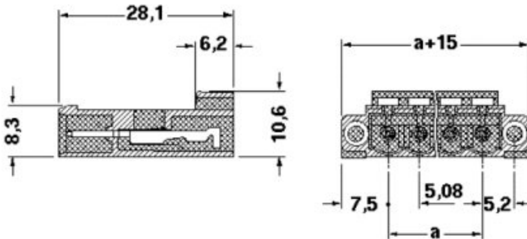
Dimensioned drawing
